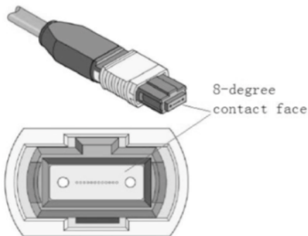
Figure 22 MTP/APC Cable
